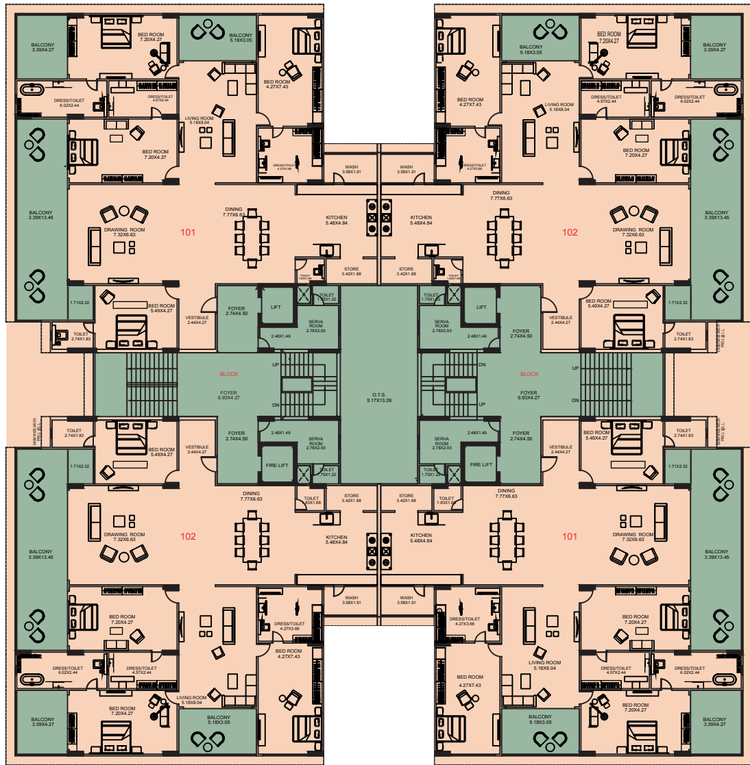
2ND to 13TH FLOOR PLAN
